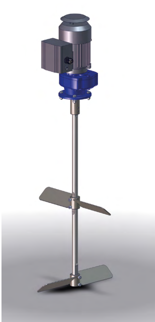
Agitator for 216.5l drum Order No. 0666355
